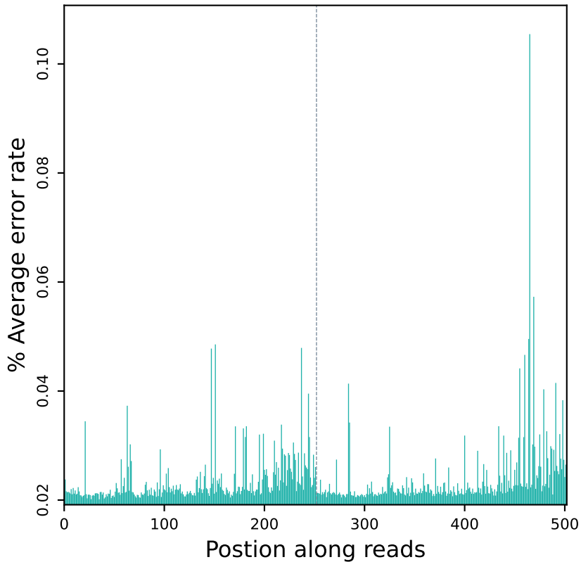
Error rate distribution along reads (R10701)
